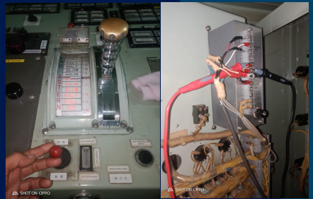
CPP control unit trouble shooting repair ( Sagita)
